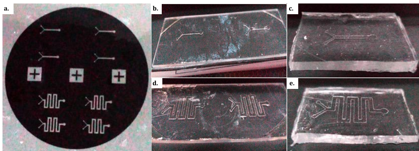
Figure 4. Design for microfluidics: (a) the overall printed photomask, (b) the SU-8 master template, and (c) the PDMS replicate of a simple Y-junction design, as well as (d) the SU-8 master template and (e) the PDMS replicate of a mixer by U-turn design.
