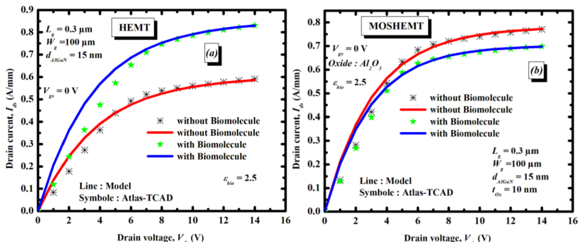
Figure 4. Comparison of the current-voltage characteristics. (a) AlGaN/GaN heterostructures based HEMT and (b) AlGaN/GaN heterostructures based MOSHEMT.
