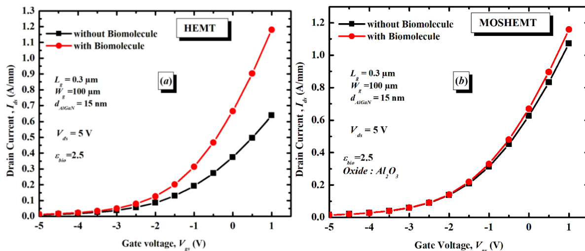
Figure 5. Comparison of the modeled I_{ds} - V_{gs} characteristics, (a) AlGaN/GaN heterostructures based HEMT and (b) AlGaN/GaN heterostructures based MOSHEMT.
