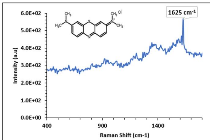
Figure 6. As-prepared macroSi-MB Raman
