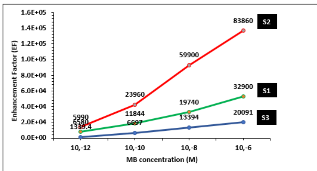
Figure 8. Relevance of enhancement factor and concentrations of MB for hybrid structures SERS sensors
