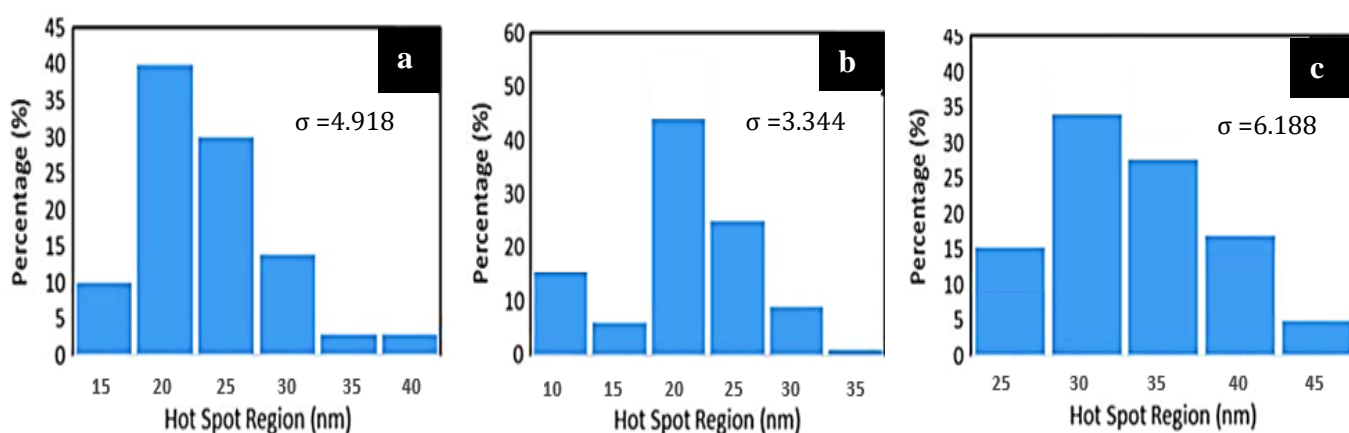
Figure 4. Histogram of hot spot regions through hybrid structures SERS sensors
