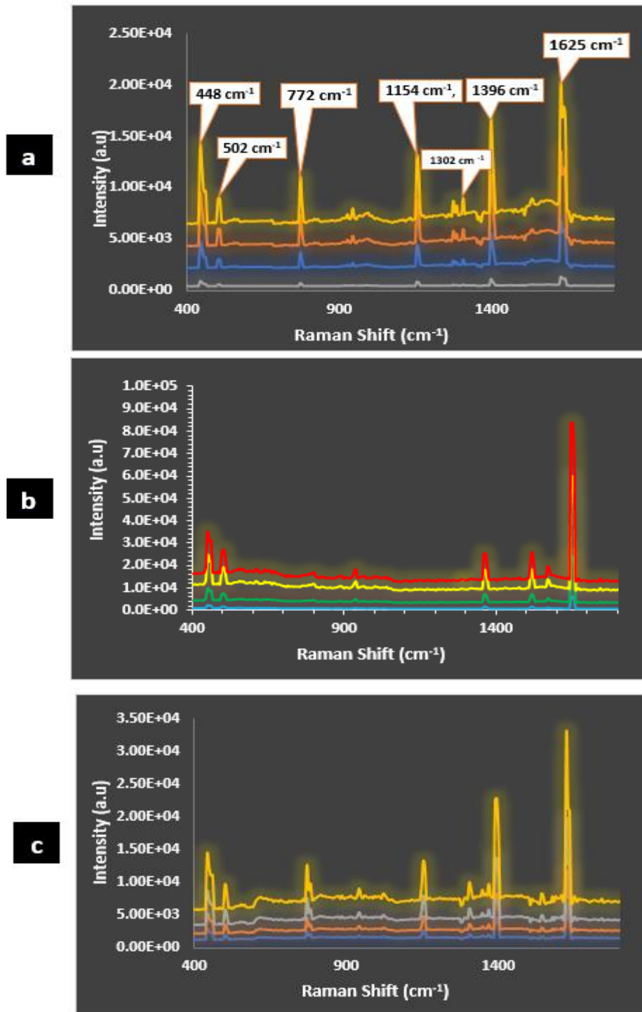
Figure 7. SERS-Spectra of hybrid structures SERS sensors
