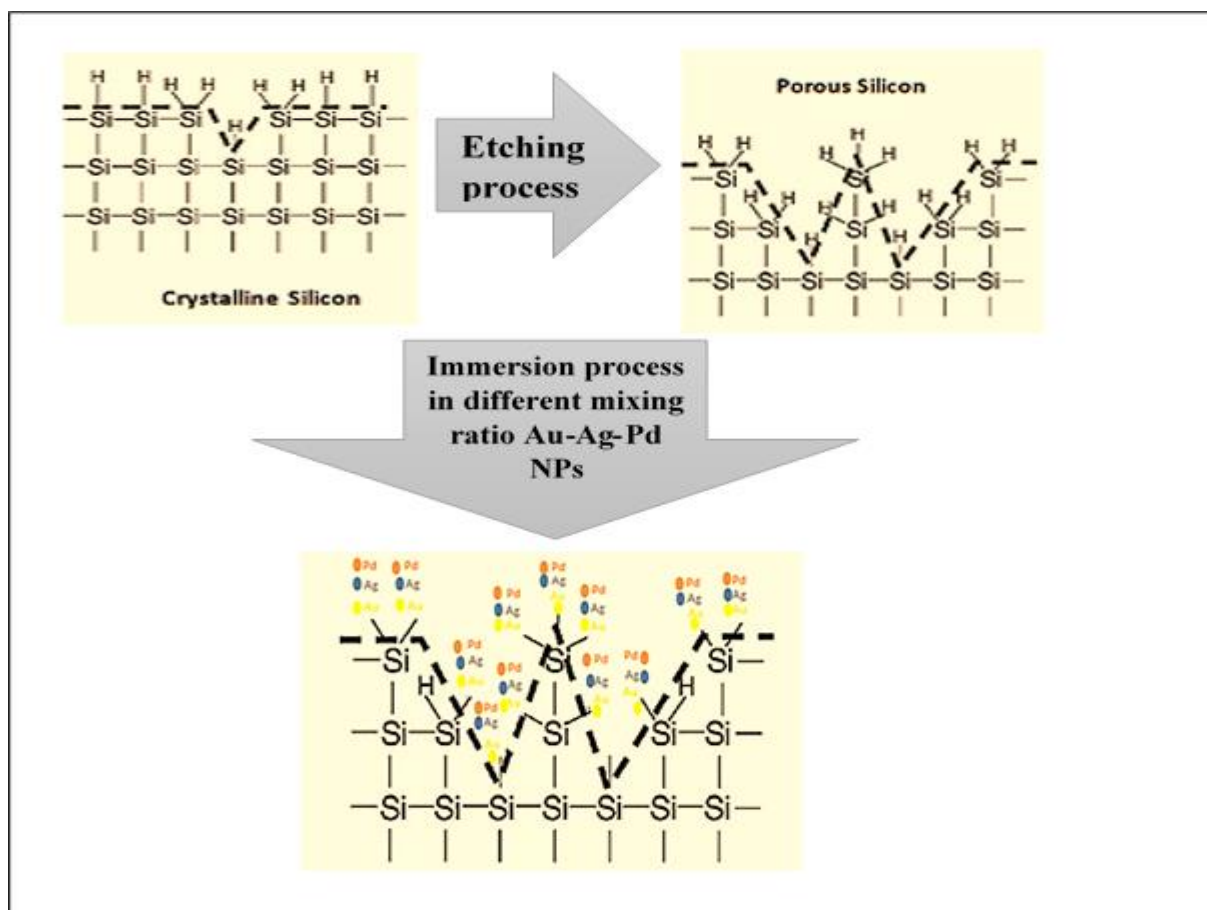
Figure1. Graphical explanation of the preparation for trimetallic surface alloy structures
