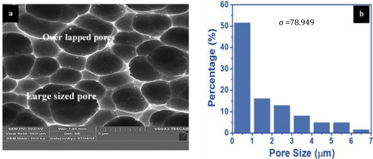
Figure 2. (a) Image of as-prep are macroPSi of FE-SEM (b) Pore volume distribution
