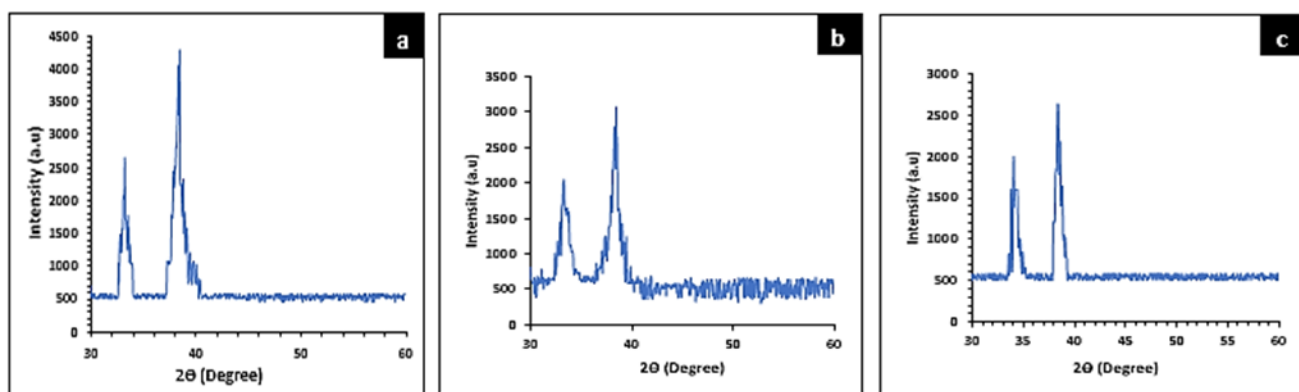
Figure 5. S.S.A-XRD style of three hybrid structures SERS sensors
