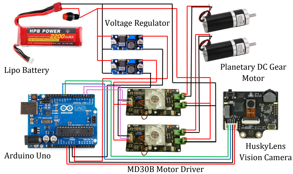
Figure 3. Electrical system
