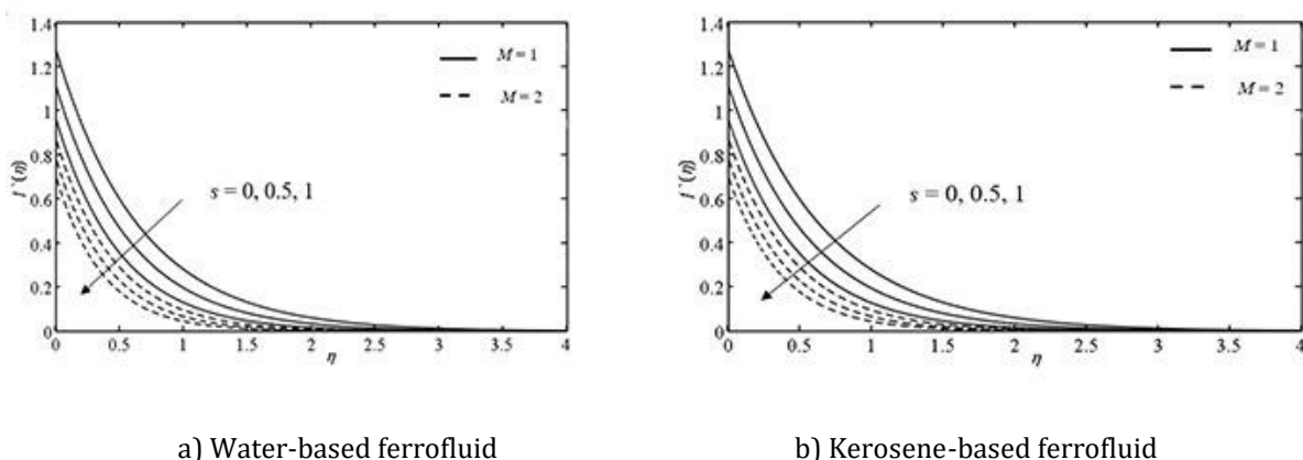
Figure 3. Effects of the suction parameter, s on velocity profiles for various M .
